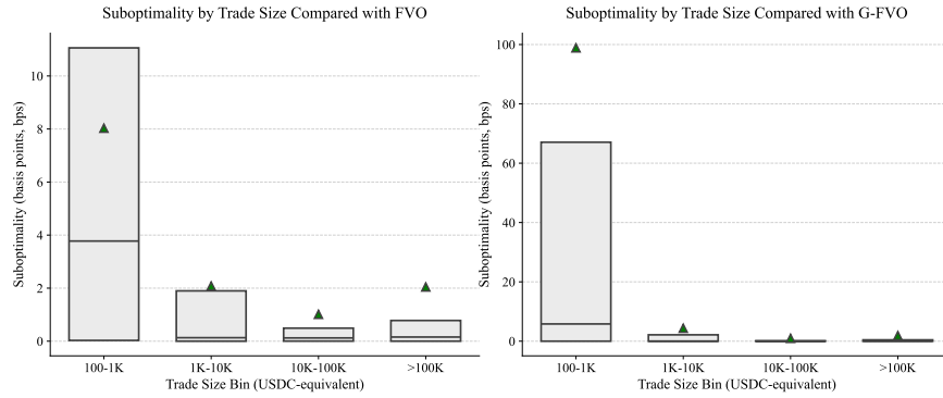
Fig. 2. Suboptimality vs. trade size (relative to FVO).
