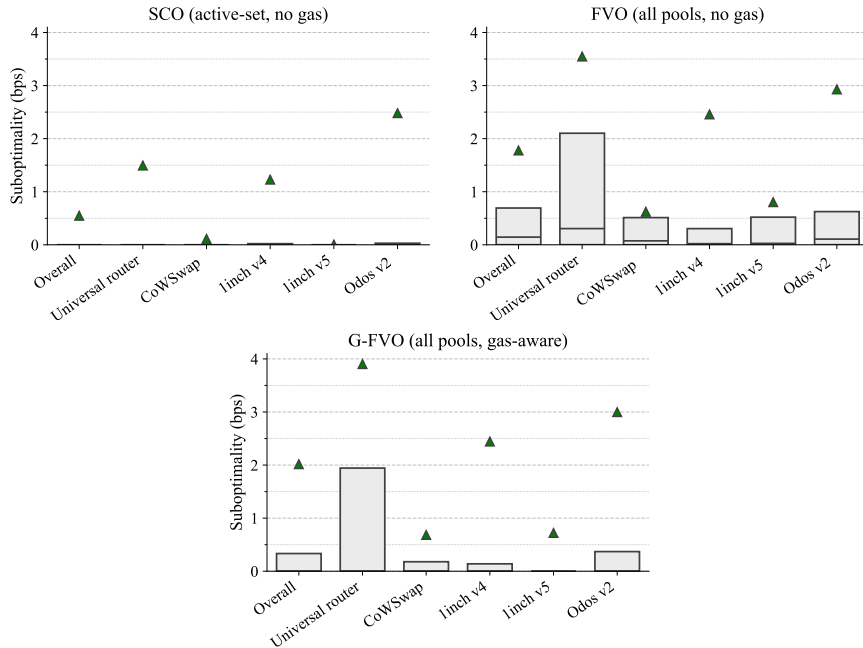
Fig. 1. Suboptimality relative to different optima. The box plot indicates the 25th, 50th, and 75th percentiles, while the triangle indicates the mean of each sample.
